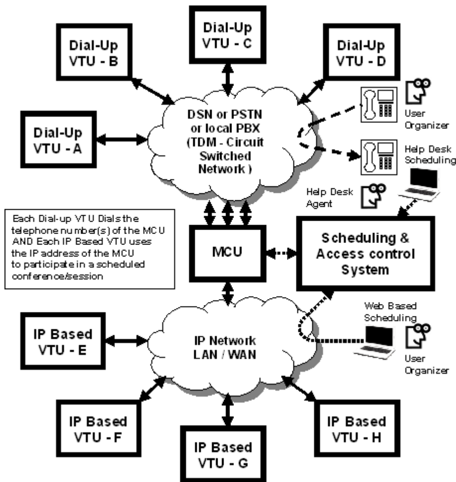
Figure 2-3: Multipoint VTC Connectivity
