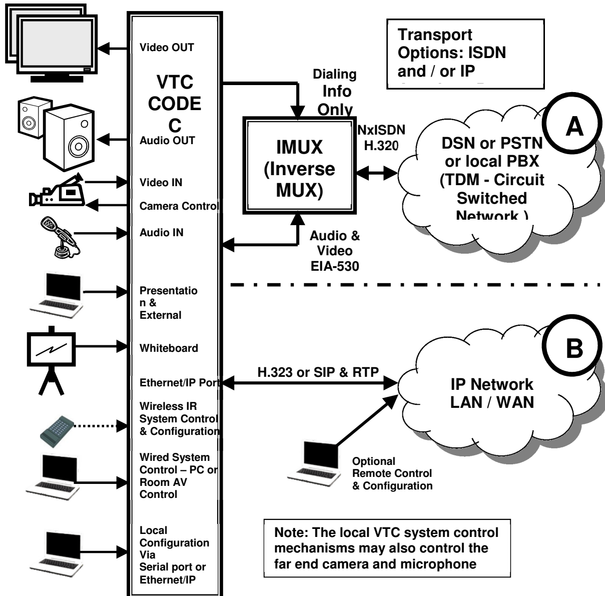
Figure 2-1: VTC Endpoint Components and Connections
